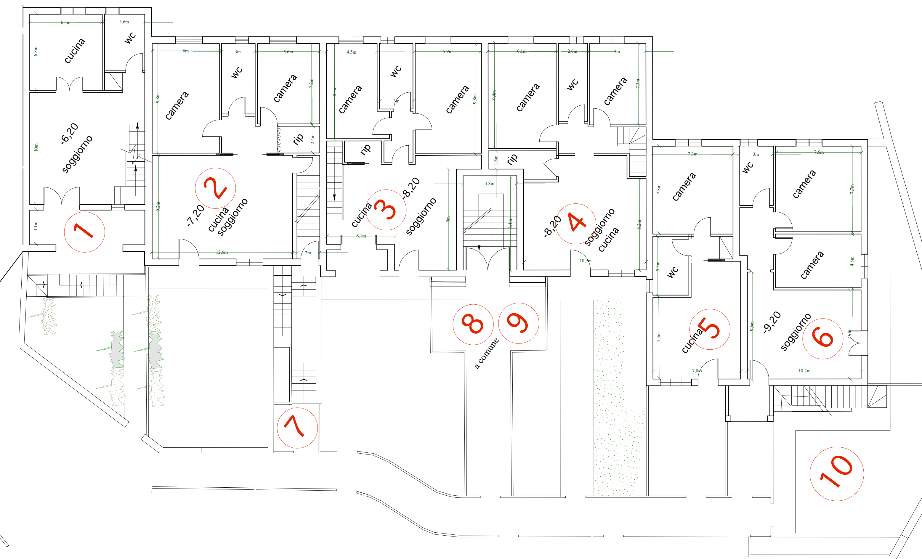
PIANO TERRENO
